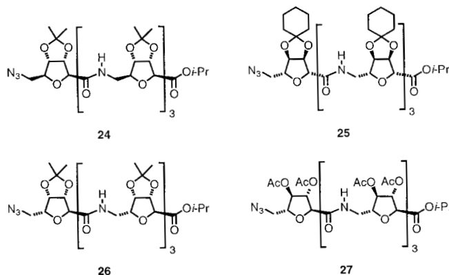
Fig. 6 Fleet's stereoisomeric tetramers from the THF-amino acid 23
