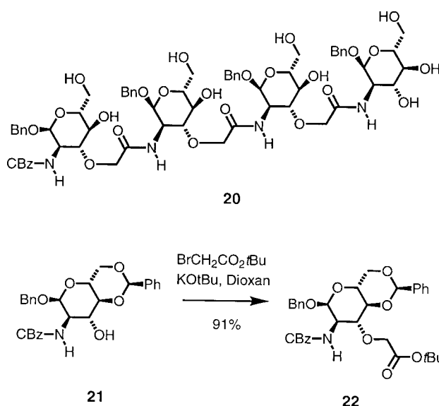
Scheme 3 A key step in the synthesis of the saccharide-peptide hybrid 20
