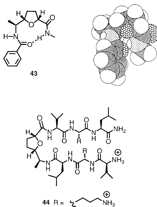
Fig. 7 \beta -Turn type solid-state structure of the THF dipeptide 43 and structure of the hairpin candidate 44
