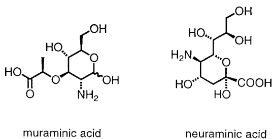
Fig. 1 Naturally occurring ether amino acids
